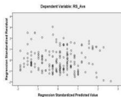
Gambar 2. Scatterplot Regression Standardized Residual terhadap Regression Standardized Predicted Value memenuhi homoskedastisitas dan linearitas
