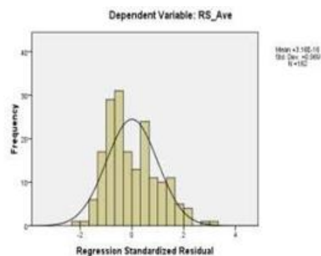
Gambar 1. Histogram uji random eror terdistribusi normal
